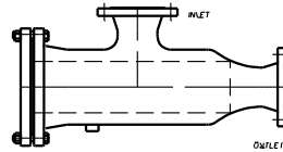
T-BODY FULL-BORE INLINE
