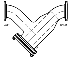
Y-BODY FULL-BORE INLINE
